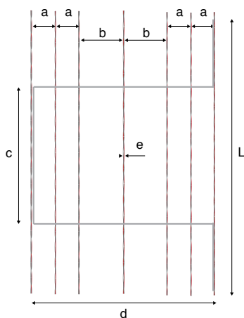
Murfor® Compact I-50
